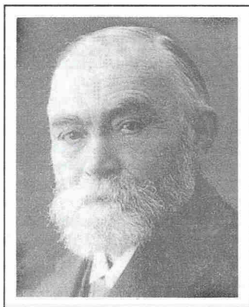
Gottlob Frege.
