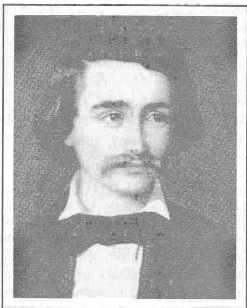
Richard Dedekind.
