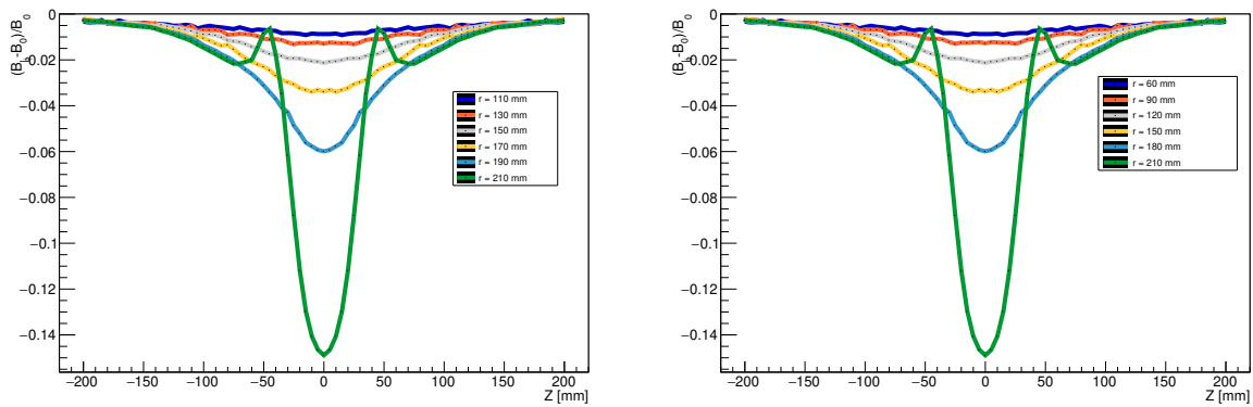
Figure A.11. Left: relative magnetic field for B_\phi with an angle of 9 degrees with drain holes, goes for radius equal to 110 to 210 mm. Right: relative magnetic field for B_\phi with an angle of 9 degrees with a deeper drain holes effect, goes for radius equal to 60 to 210 mm. In both plots the X axis represents the beam axis ( Z ), where the zero is the center of the drain hole.
