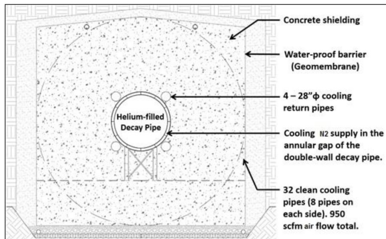
Figure 5.10. Schematic of decay pipe design for LBNF. Image taken from [30].
