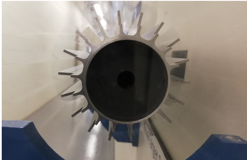
Figure 3.4. Baffle for NuMI beam.
