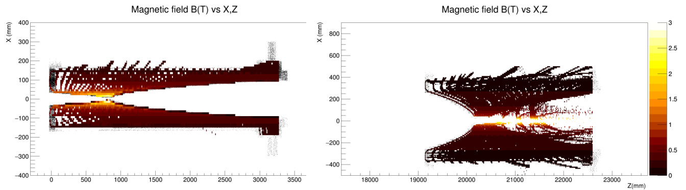
Figure 6.2. Left: Magnetic field in Horn 1 of NuMI beam simulation. Right: Magnetic field in Horn 2 of NuMI beam simulation.
