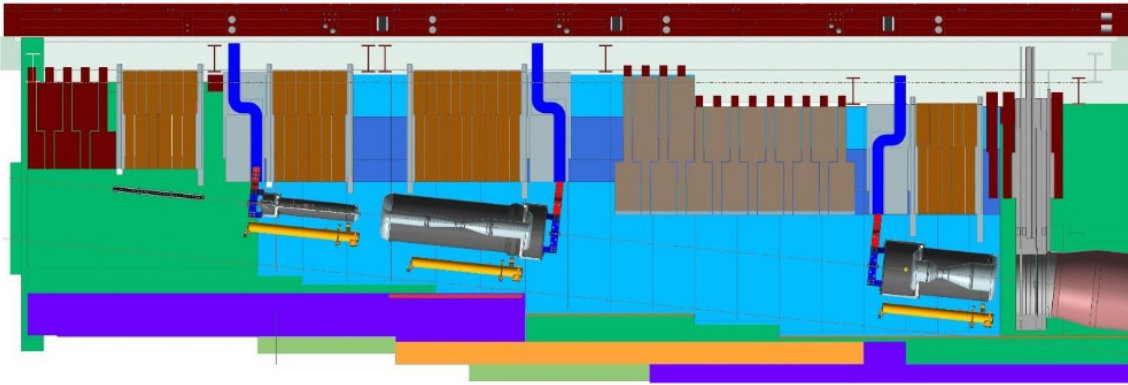
Figure 5.3. Schematic of LBNF neutrino beam, from left to right baffle, 3 focusing horns and the decay pipe. Image taken from [30].
