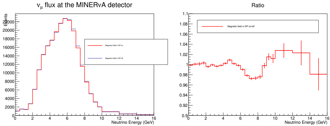
Figure 6.17. Left: \nu_\mu flux at the center of the MINER \nu A detector, the red one corresponds to magnetic field on, and the blue one to magnetic field off. Right: Ratio of \nu_\mu flux at the center of the MINER \nu A detector, magnetic field ON/OFF on decay pipe. Obtained with the nominal simulation of NuMI beam on Geant4.
