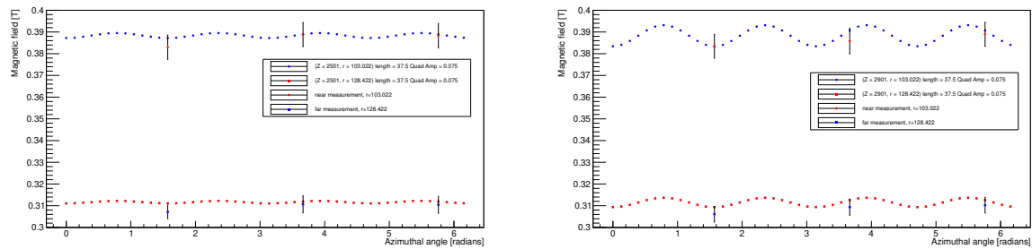
Figure A.8. Comparison between the measurement and length scale = 37.5, quadrupolar amplitude = 0.075 on water port L (left) and water port O (right).
