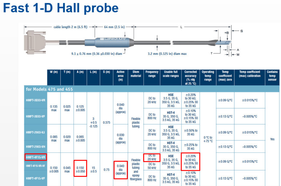
Figure 6.5. Specifications for hall probe used to measured the B field. Image taken from [35].
