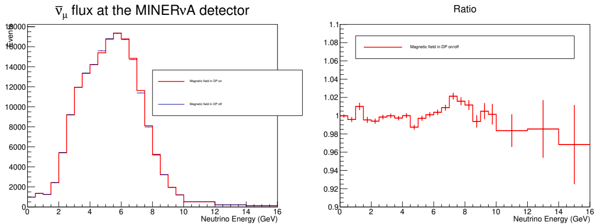
Figure 6.18. Left: \bar{\nu}_\mu flux at the center of the MINER \nu A detector, the red one corresponds to magnetic field on, and the blue one to magnetic field off. Right: Ratio of \bar{\nu}_\mu flux at the center of the MINER \nu A detector, magnetic field ON/OFF on decay pipe. Obtained with the nominal simulation of NuMI beam on Geant4.
