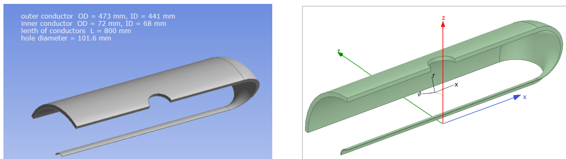
Figure 7.2. Left: a quarter of horn A of LBNF simulated on ANSYS, the hole diameter equal to 101.6 mm. Right: Coordinate system for ANSYS simulation, the coordinate system is different that the used for Geant4 simulation. Images taken from [36].
