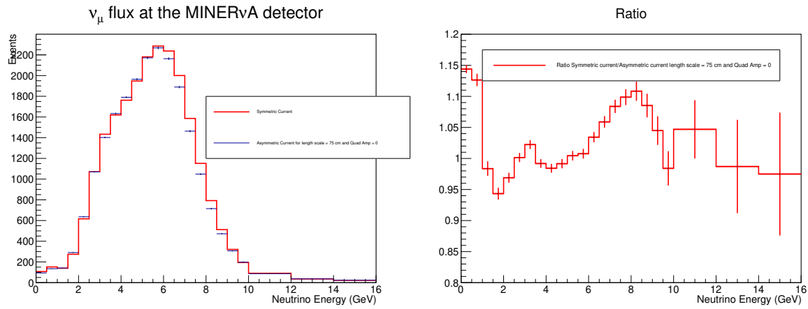
Figure A.7. Left: Histogram of \nu_\mu flux at the center of the MINER \nu A detector, nominal simulation on red, CEQ length scale = 75 and quadrupolar amplitude equal to 0.0 on blue. Right: Ratio of \nu_\mu flux at the center of the MINER \nu A detector, nominal simulation over CEQ length scale = 75 and quadrupolar amplitude equal to 0.0. The simulation is broken, can not be trusted for this length scale.
