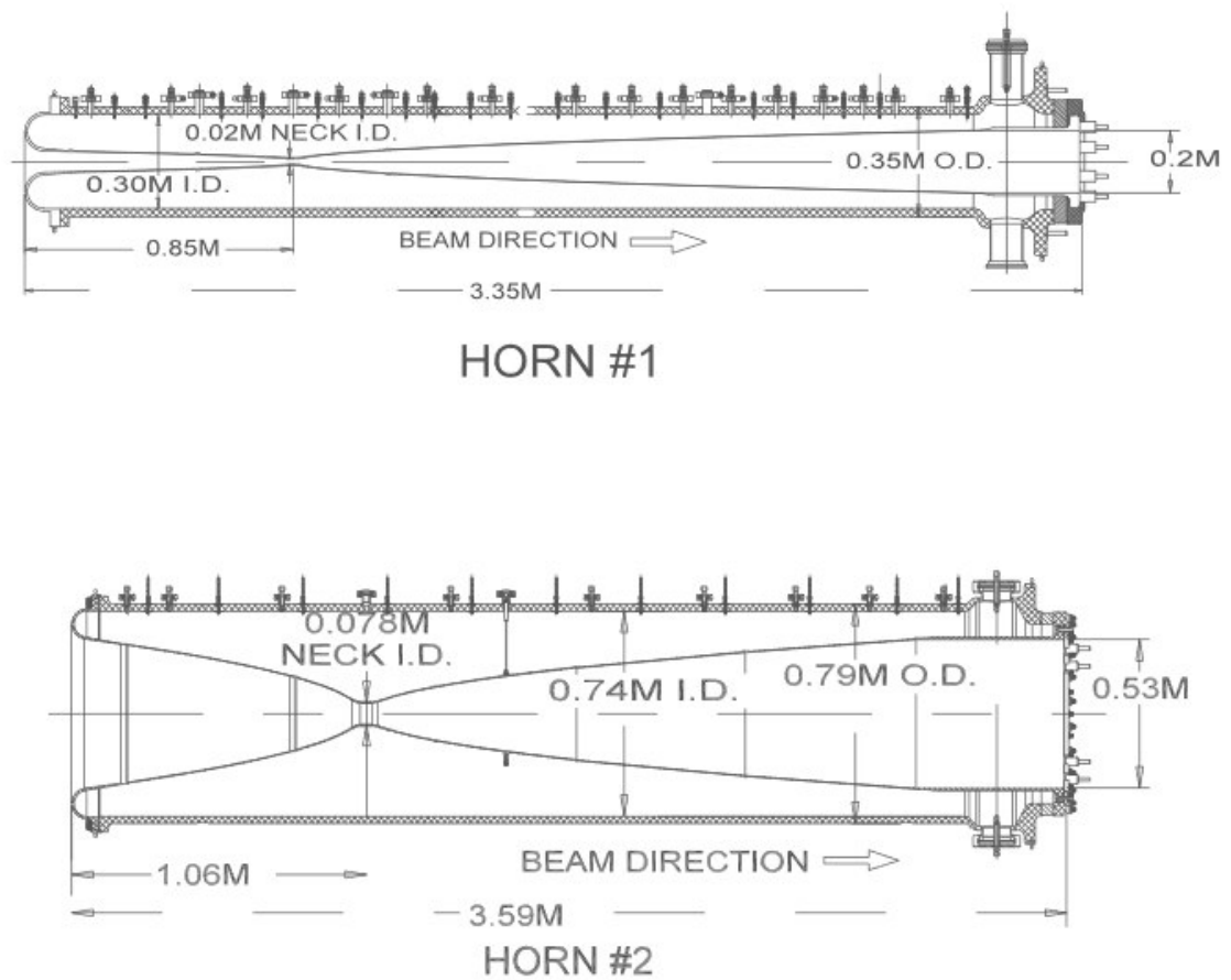
Figure 3.8. Schematic of NuMI magnetic horns. Image taken from [6].
